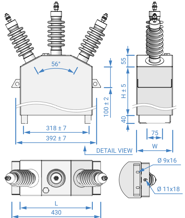
CUFFS - Single phase type, live case
