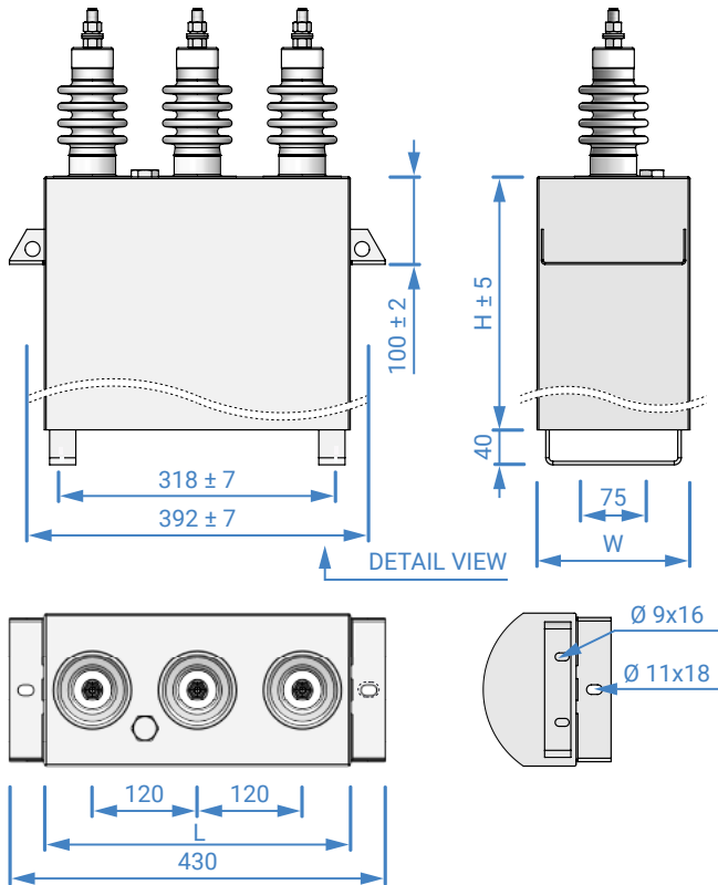
CPEFS - Three phase unit, up to 12kV
