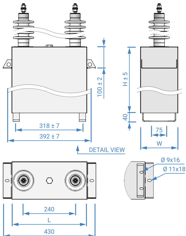
CUEFS - single phase type, insulated case
